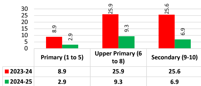
Dropout Rate
